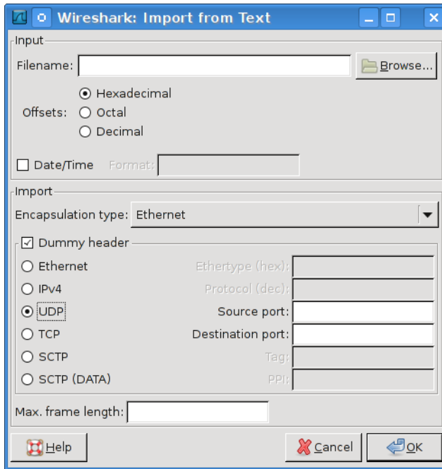
Figure 5.10. The "File Import" dialog
