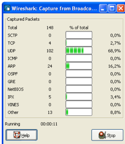
Figure 4.13. The "Capture Info" dialog box
